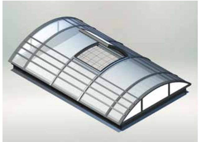
plus arcade rooflight with ID600, EAD and 1 m apex vent with ventilation function
